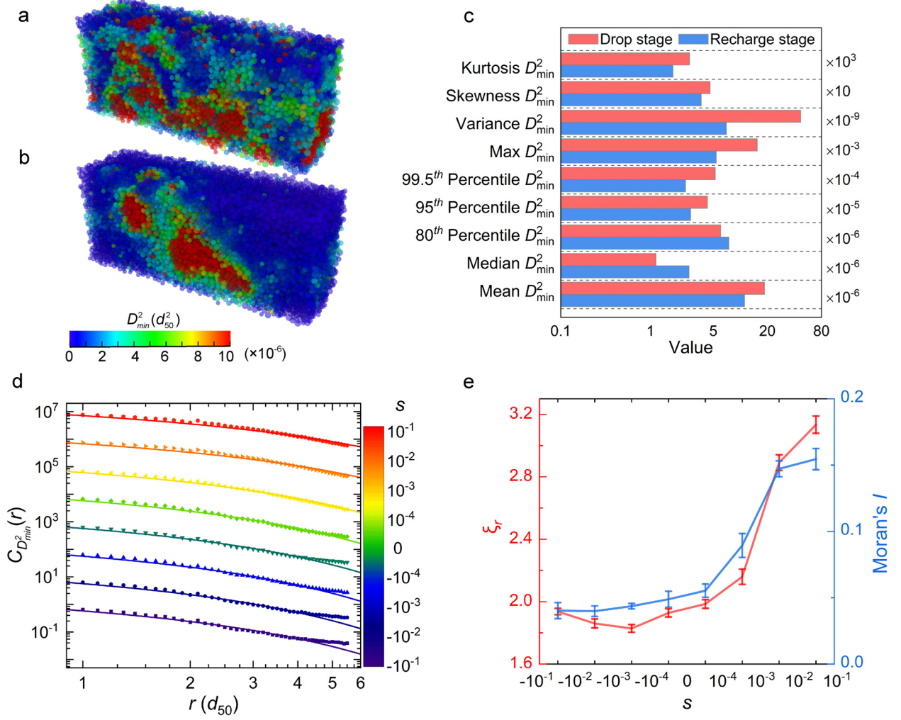
Fig. 3. Statistical and spatial characteristics of microslips occurred during recharge and drop stages. Spatial maps of D_{min}^2 occurred during the (a) recharge stage and (b) drop stage of a typical stick-slip cycle. (c) Comparison of the statistical quantities of D_{min}^2 during the recharge and drop stage. (d) Normalized spatial correlation function of D_{min}^2 : C_{D_{min}^2}(r) between two particles separated by distance r , where r is in unit of the mean particle diameter. The data points are averaged over the recharge or drop stages falling into each bin. Solid lines are fits to the Ornstein-Zernike function. The data points and fitting lines of the different bin are shifted vertically for better visualization. (e) Evolutions of correlation length \xi_r and Moran' I with the magnitude of stress fluctuation. The error bar represents the standard deviation. Note that (d) and (e) are calculated over all stick-slip cycles.
