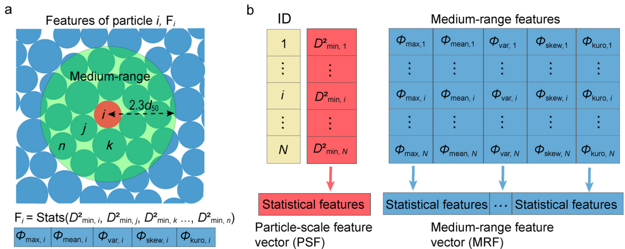
Fig. 4. Machine learning builds the bridge between microslips and macroscopic stress fluctuation. (a) The statistical characteristics of particle D_{min}^2 within each particle's second-neighbor shell. (b) Feature extraction process: particle-scale feature vector (red column) and medium-range feature vector (blue columns). These two feature vectors are fed as input to the downstream XGBoost model to predict macroscopic stress fluctuation.
